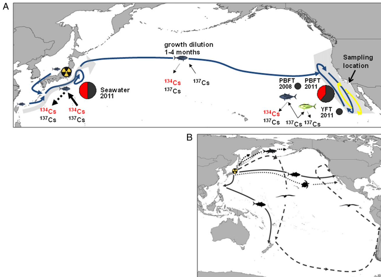
Fig. 1. (A) Map of the northern Pacific ocean showing simplified movement patterns for juvenile PBFT (blue arrows) from Japan to the CCLME and juvenile YFT (yellow arrows) in the CCLME. Kuroshio Current (gray arrow east of Japan) and CCLME (gray region west of N. America) are shown. Pie charts show mean concentrations of ^{134}\text{Cs} (red) and ^{137}\text{Cs} (dark gray) in seawater (Bq m ^{-3} ) (3), and muscle tissue (Bq kg ^{-1} ) in PBFT after Fukushima, PBFT before Fukushima, and YFT after Fukushima. Pie charts for fish are sized to scale of total radiocesium concentrations. Black arrows show uptake (solid arrows) and efflux (dotted arrows) of radiocesium in different ocean regions (arrow thickness scaled for relative efflux and uptake rates). (B) Simplified migration patterns of some highly migratory species in the Pacific that inhabit waters around Japan and make subsequent long distance migrations to distant ecoregions including Kamchatka, the Aleutian Islands, North America, South America, and New Zealand. Migration patterns are shown for salmon sharks (17) (short dashed line), sooty shearwaters (18) (long dashed line), Pacific bluefin tuna (6) (solid lines), and loggerhead turtles (19) (dotted line).
