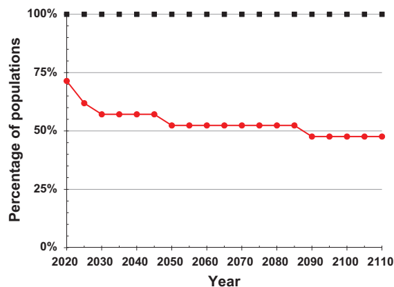
Figure 3 Percentage of populations expected to persist at densities > 10% of their potential in the future. Differences between fenced (black squares, n = 16 ) and unfenced (red circles, n = 21 ) reserves each year are all significant by Fisher test.
