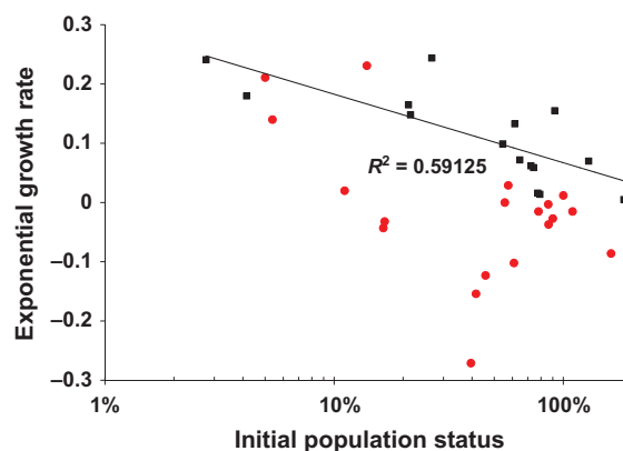
Figure 2 Effect of population density on population growth rate over the following 10 years for fenced (black) and unfenced (red) reserves. 'Initial population status' refers to the observed population density at the start of each time series compared to the expected density. The black regression line is for fenced reserves.
