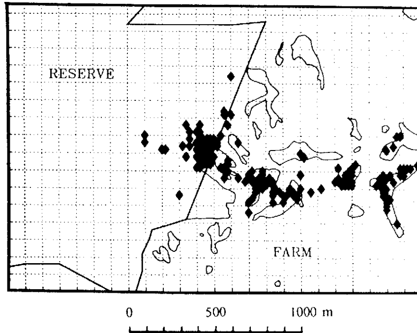
Location records for a female Brown Kiwi at Paerata Wildlife Management Reserve illustrating the use of a number of stepping stone remnants outside the reserve boundary. From Potter (1990) with permission, New Zealand Ecological Society.
