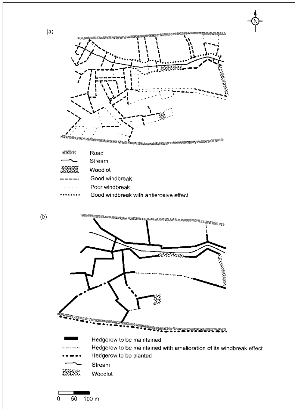
Fig. 9-11 Diagrams of a hedgerow network in Campénéac, France, (a) before “remembrement” and (b) the design that ecologists recommended for retention. Redrawn from Baudry and Burel (1984) with permission, Elsevier Science-NL.
